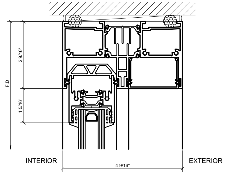
⑤ HEAD AT FIXED PANEL 1'-0"=1'-0" ARCH REF: N/A
